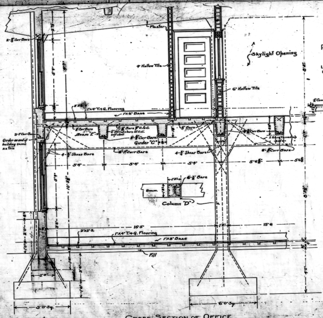
CROSS SECTION OF OFFICE SCALE 1/2" = 10'
